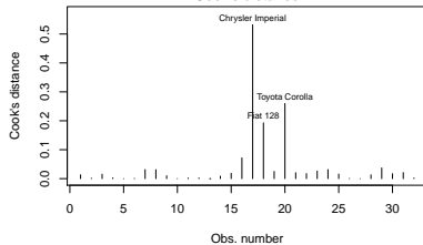
Cook's distance
